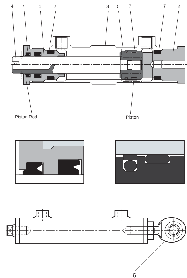
Figure 6 32mm dia. Piston
