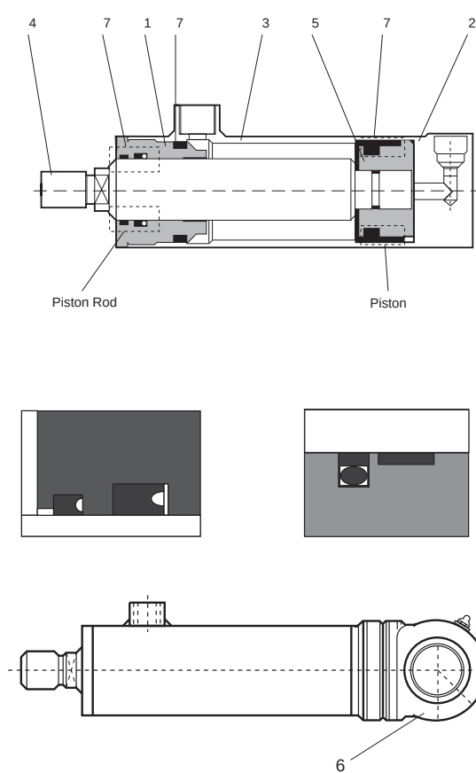
Figure 7 40mm to 63mm dia.bore
